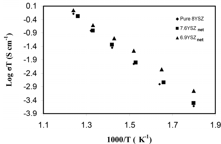
Fig. 8. Temperature dependence of total conductivity of 6.9YSZ net sample before and after annealing
