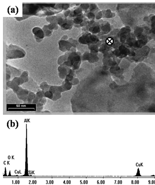
Fig. 8. (a) BFI of Al-5%SiC nanocomposite powder obtained after 25 h of ball-milling and (b) EDS analysis of the region marked in (a).
