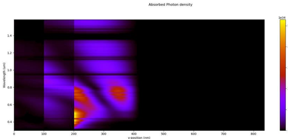
Fig. 18. Absorbed photon density in the Perovskite solar cell
