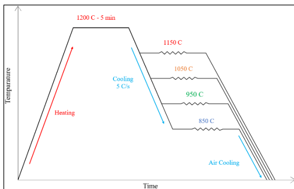
Fig. 1. Schematic diagram of the hot compression process
