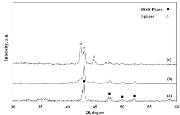
Fig. 5. The XRD patterns of Mn_{50}Al_{50} milled sample after the annealing process at 500°C for a) 30, b) 90 and c) 180 min.
