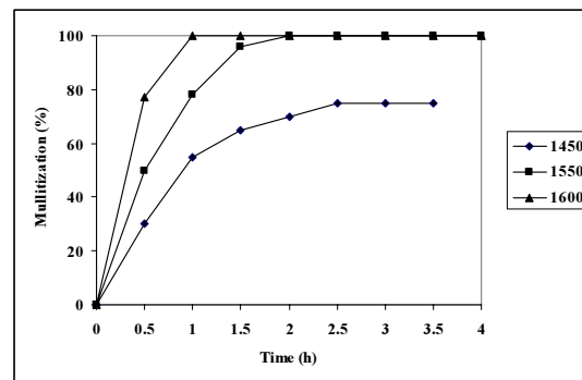
Fig. 5. Results of mullitization versus the soaking time at different temperatures with 38 μm in size for kyanite concentrate
