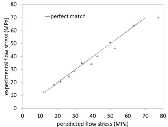
Fig. 7. Correlation between experimental and predicted flow stresses of studied Al 6061 alloy.
