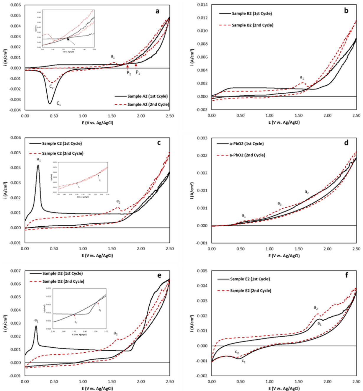
Fig. 1. Cyclic voltammetry of Ti substrate in 0.1 M \text{HNO}_3 , 0.5 M \text{Pb}(\text{NO}_3)_2 and a) Sample A2, b) Sample B2, c) Sample C2, d) saturated PbO in 3.5 M NaOH, e) Sample D2, f) Sample E2
