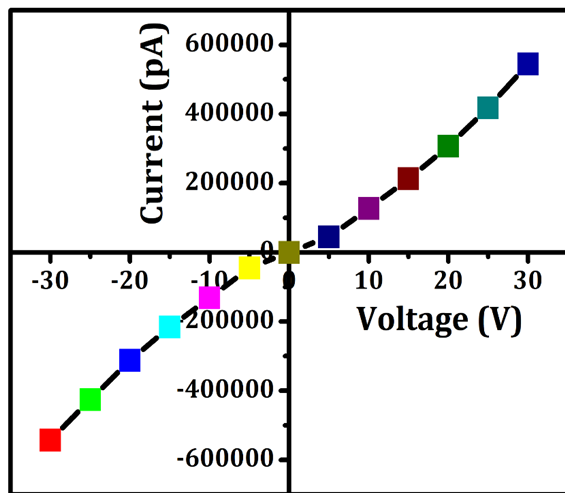
Fig. 8. I-V characteristics
