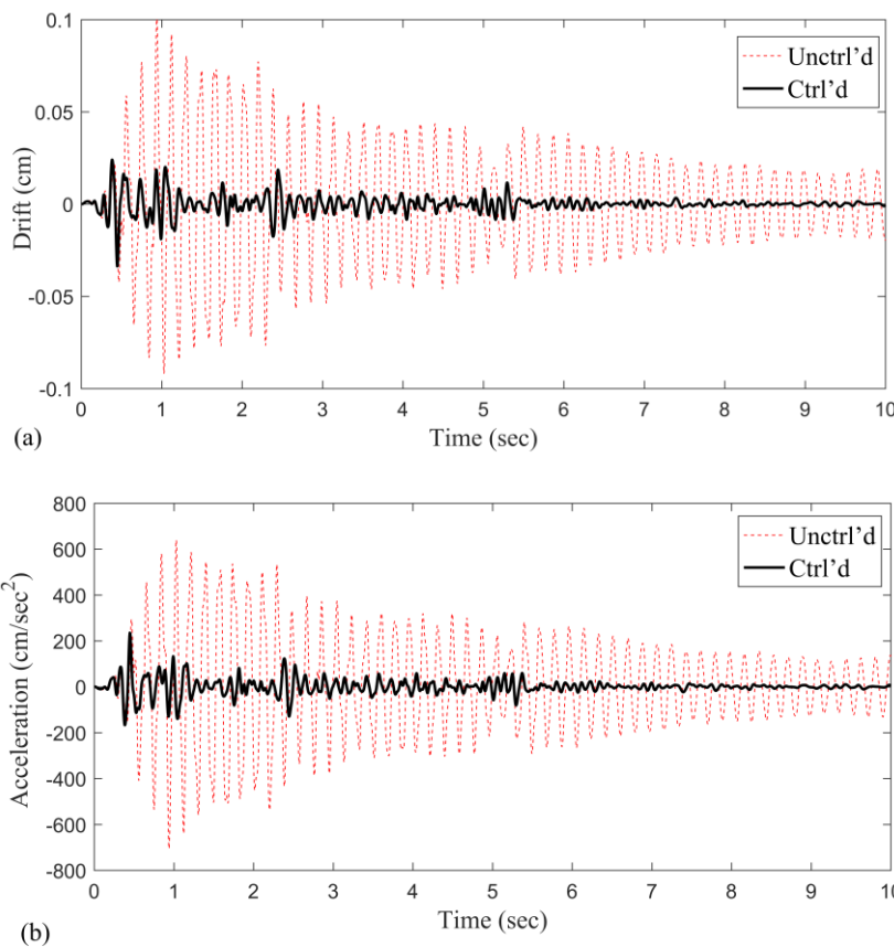
Figure 8. Time histories of responses on the third floor under the low (50%) El Centro earthquake: (a) drift; and (b) acceleration
